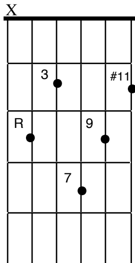
CMaj9#11
